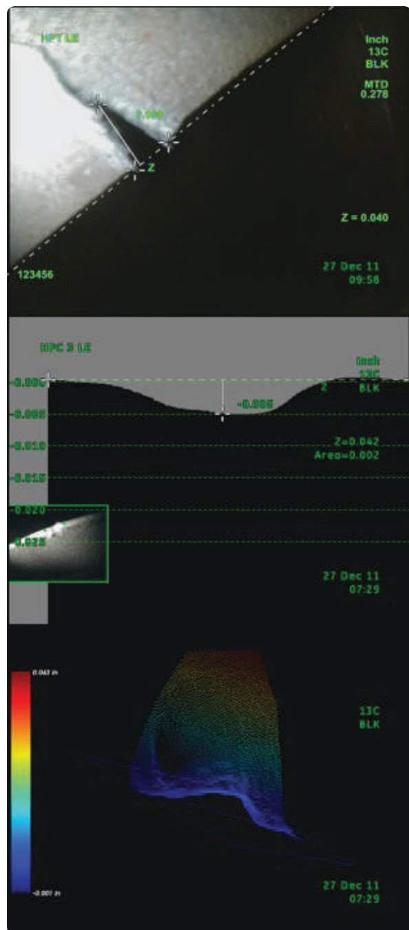
Figure 21-5. Boreoscope images.
