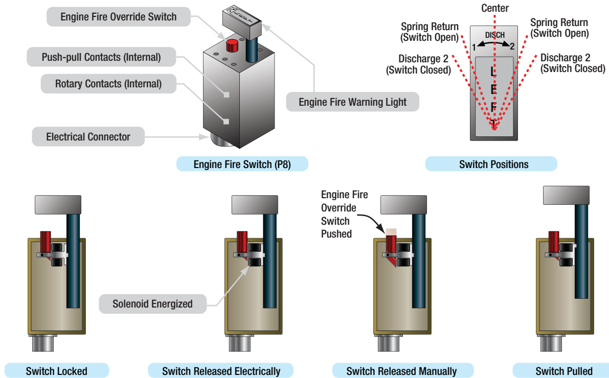
Figure 20-13. Engine fire switch operation.
