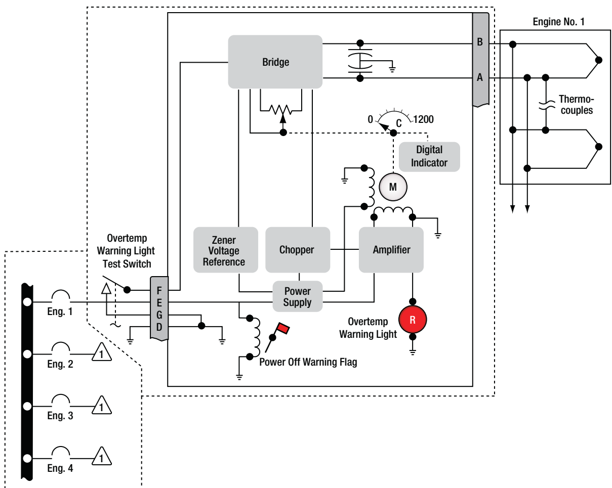
Figure 14-3. A typical analog turbine inlet temperature indicating system.
