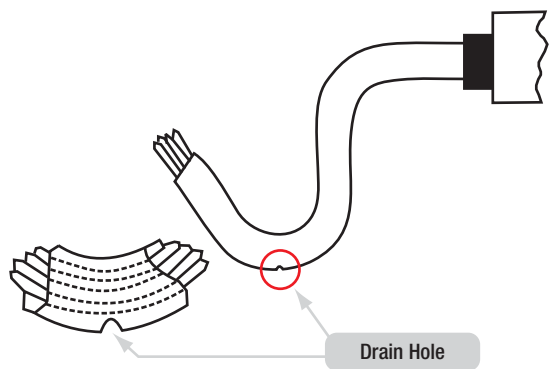
Drainage hole 1/8 inch diameter at lowest point in tubing. Make the hole after installation is complete and lowest point is firmly established.
