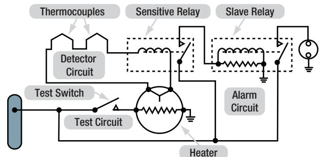
Figure 20-2. Thermocouple fire warning circuit.
