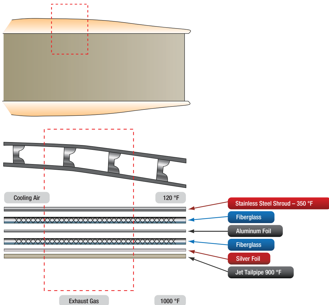
Figure 7-3. Insulation blanket with the temperatures obtained at the various locations shown.
