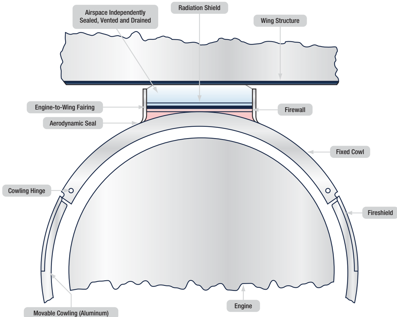
Figure 19-1. Engine firewall.
