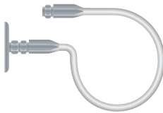
Figure 19-9. Proper hose installation.
