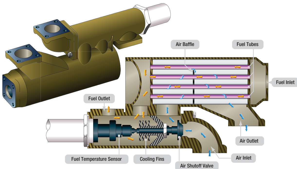
Figure 11-13. Fuel heater.
