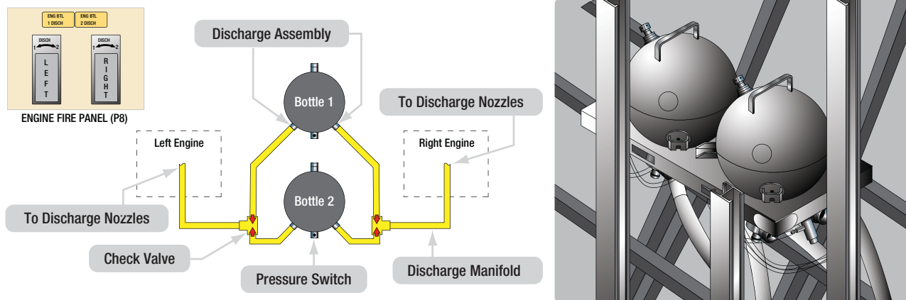
Figure 20-18. Location of fire extinguishing bottles.
