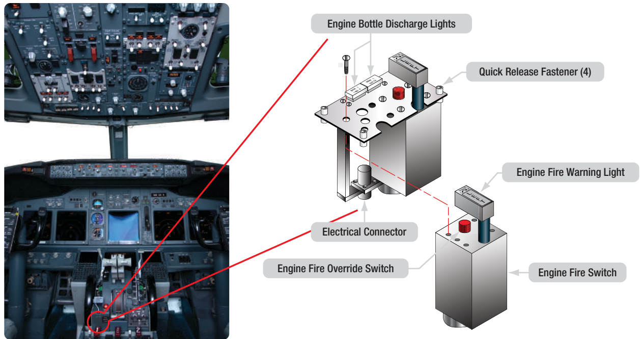
Figure 20-20. Fire switch.
