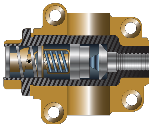
Figure 10-11. Typical thermostatic bypass valve.
