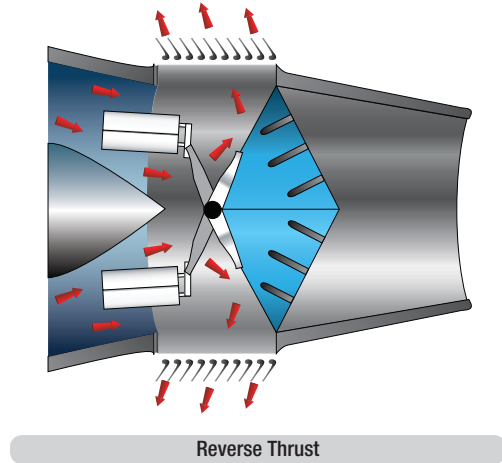
Figure 7-8. Engine exhaust gases are blocked and diverted in a reverse direction during thrust reversal.
