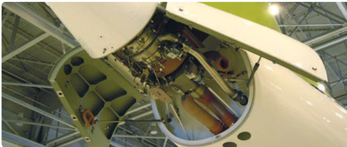
Figure 18-5. typical empennage/tail cone APU installation.
