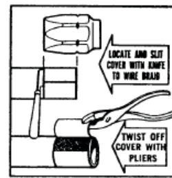
2. Locate length of hose to be cut off and slit cover with knife to wire braid. After slitting cover, twist off with pair of pliers. (see note below)
