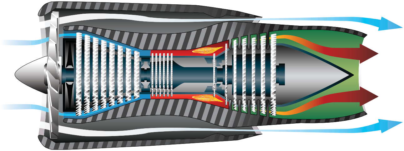
Figure 1-8. Fan airflow and core airflow of a turbofan engine.
