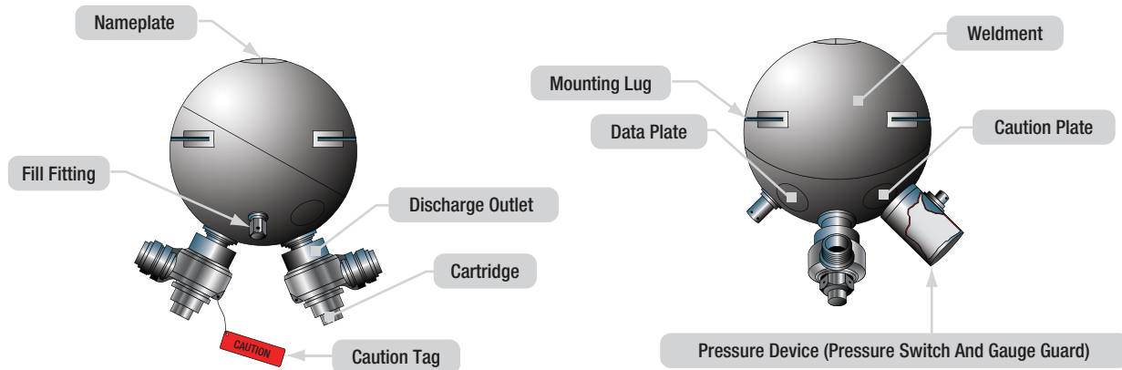
Figure 20-9. Fire extinguisher containers (HRD bottles).
