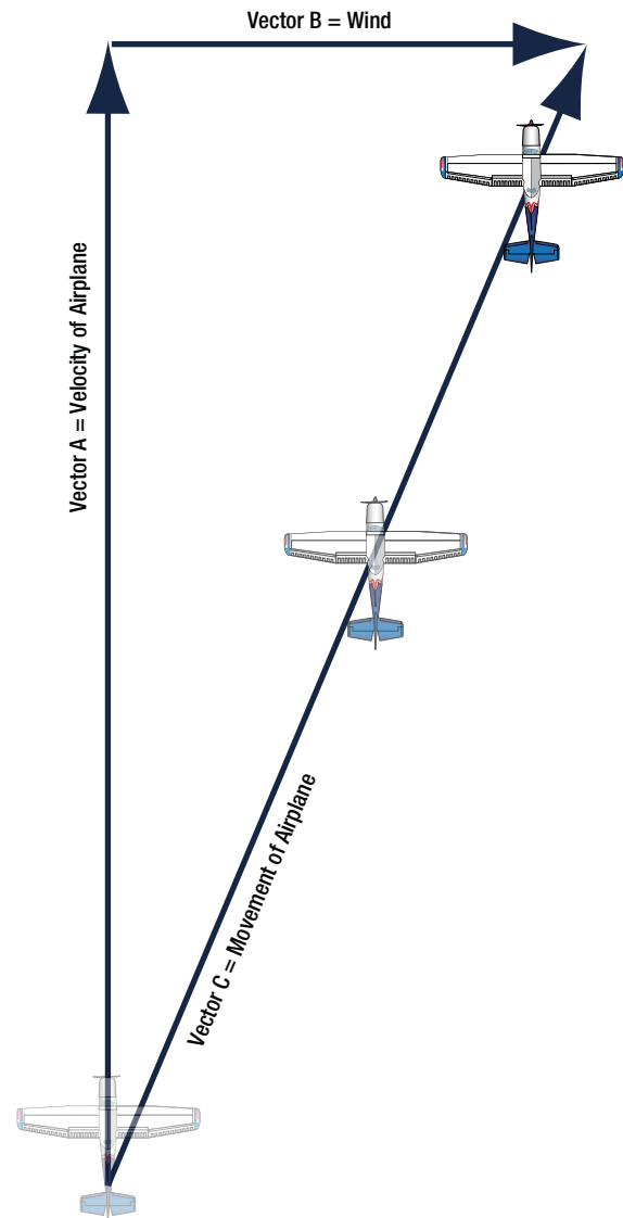
Figure 1-6. Vector analysis for airplane velocity and wind velocity.
