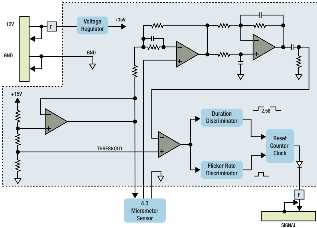
Figure 20-3. Optical fire detection system circuit.
