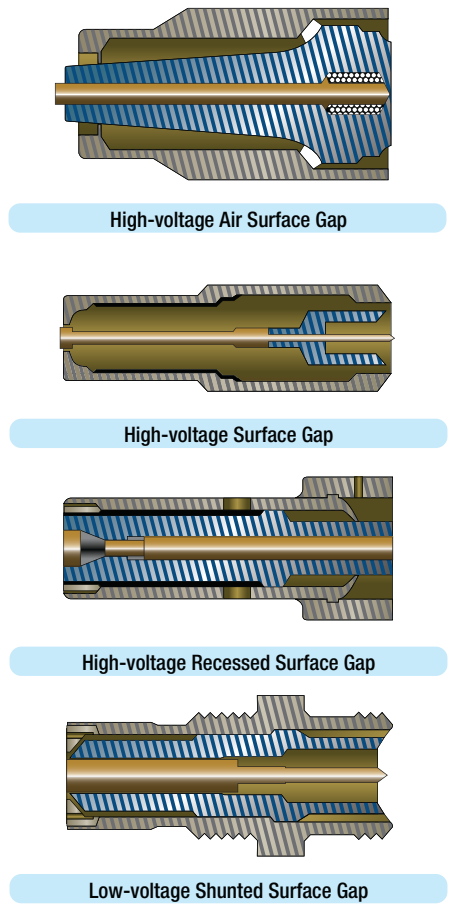
Figure 13-16. Igniter plugs.
