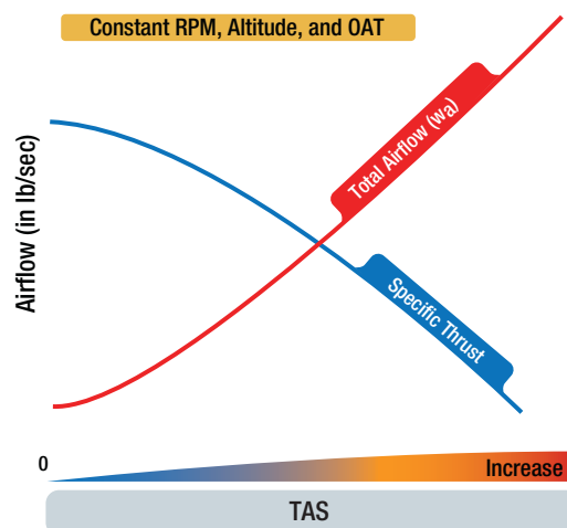
Figure 2-9. Effect of airspeed on specific thrust and total engine airflow.
