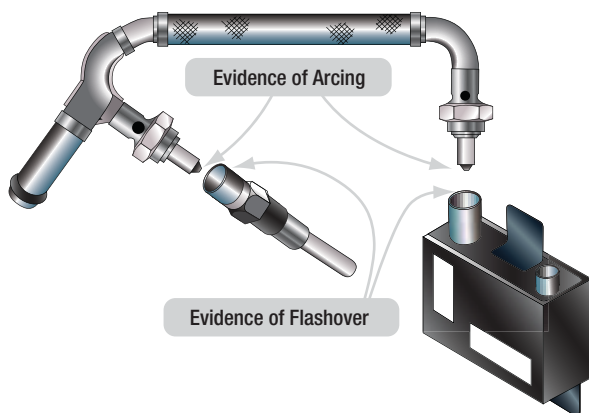
Figure 13-19. Flashover inspection.
