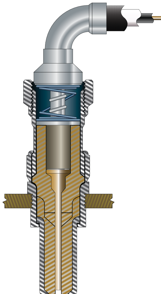
Figure 13-18. Constrained gap igniter plug.
