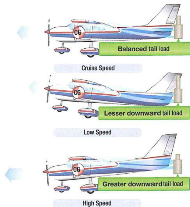
Figure 4-5. Effect of speed on downwash.
