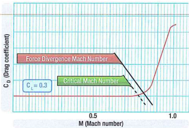
Figure 3-10. Critical Mach.
