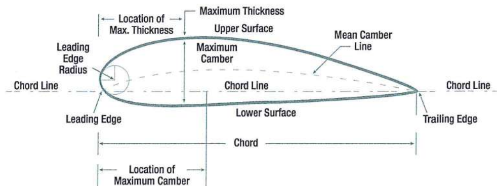
Figure 2-9. Chord and camber of a wing.
