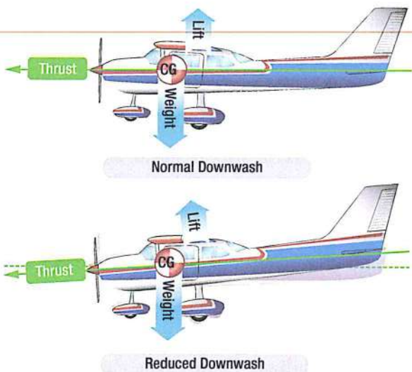
Figure 4-6. Reduced power allows pitch down.
