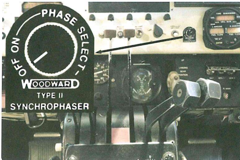
Figure 4-4. Propeller synchrophaser control.
