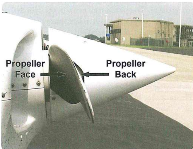
Figure 2-11. Propeller face and back.
