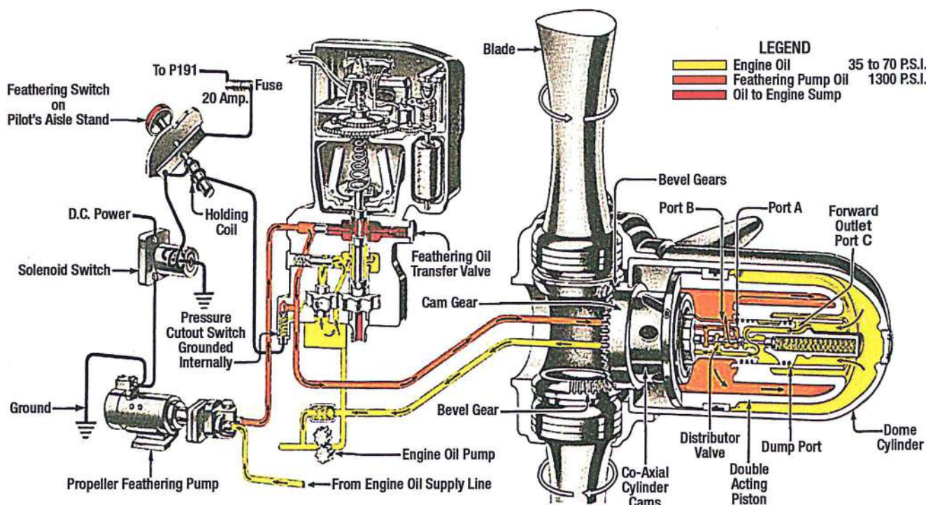
Figure 3-17. Hydromatic propeller feathering.
