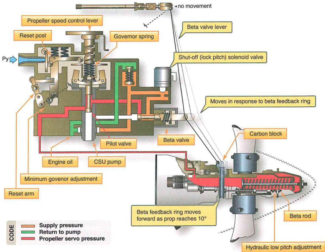
Figure 3-26. PT-6 Beta mode forward operation.
