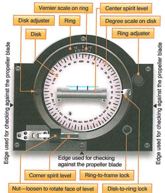
Figure 6-8. Universal protractor.
