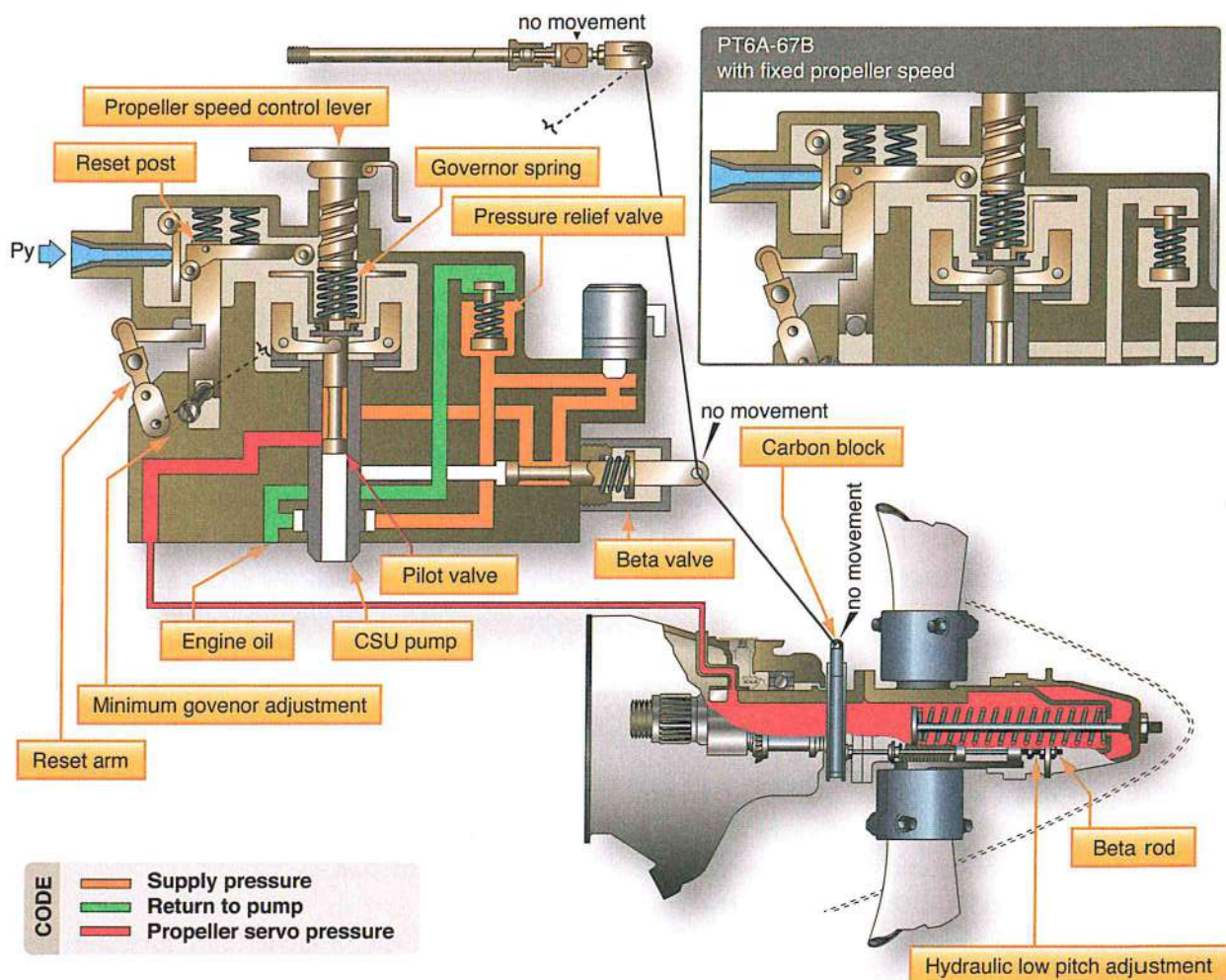
Figure 3-25. PT-6 Governing schematic.
