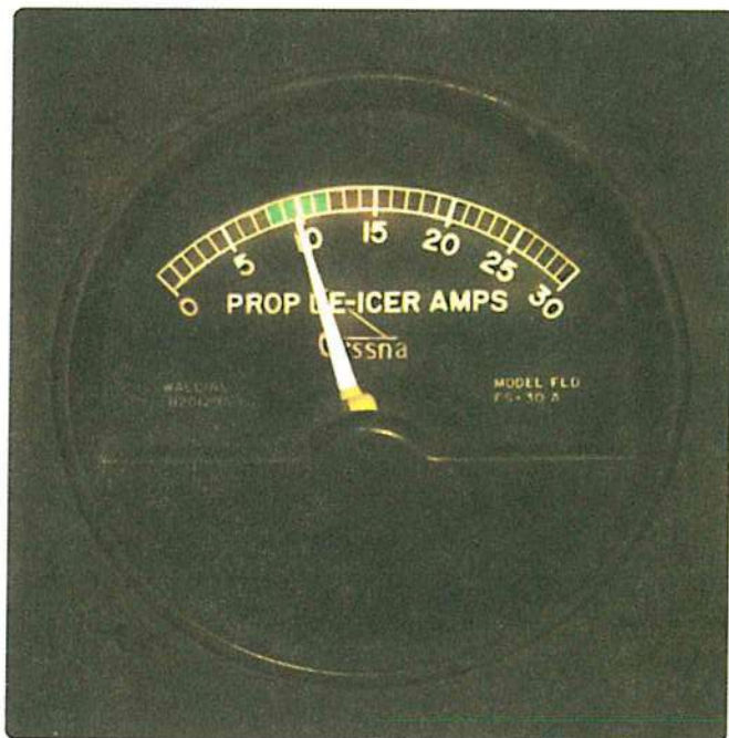
Figure 5-9. Propeller de-icer ammeter. Heating elements should draw green arc current.
