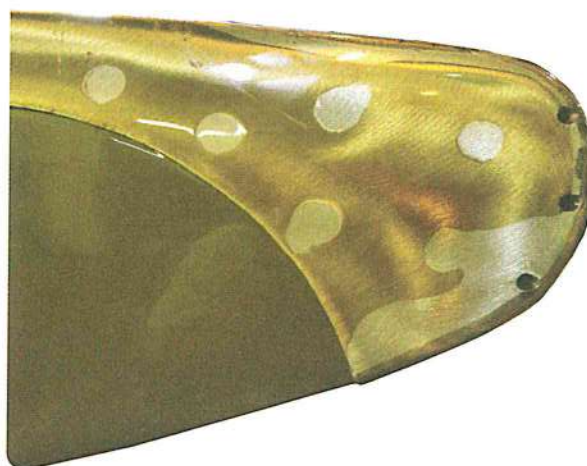
Figure 2-5. Tip on wooden propeller revealing soldered attachment hardware and drain holes.
