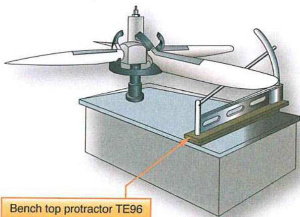
Figure 6-6. Blade angle measurement with bench-top protractor.
