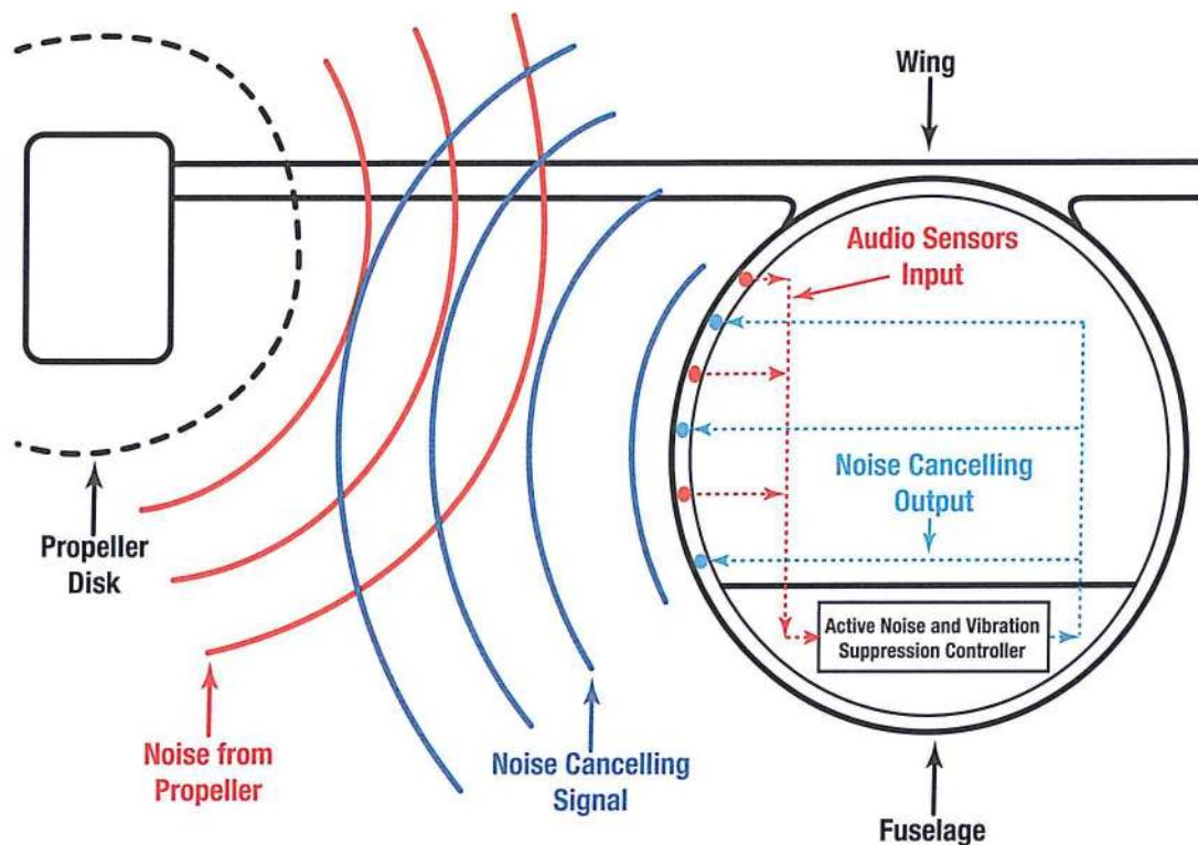
Figure 4-6. Active noise and vibration suppression system.
