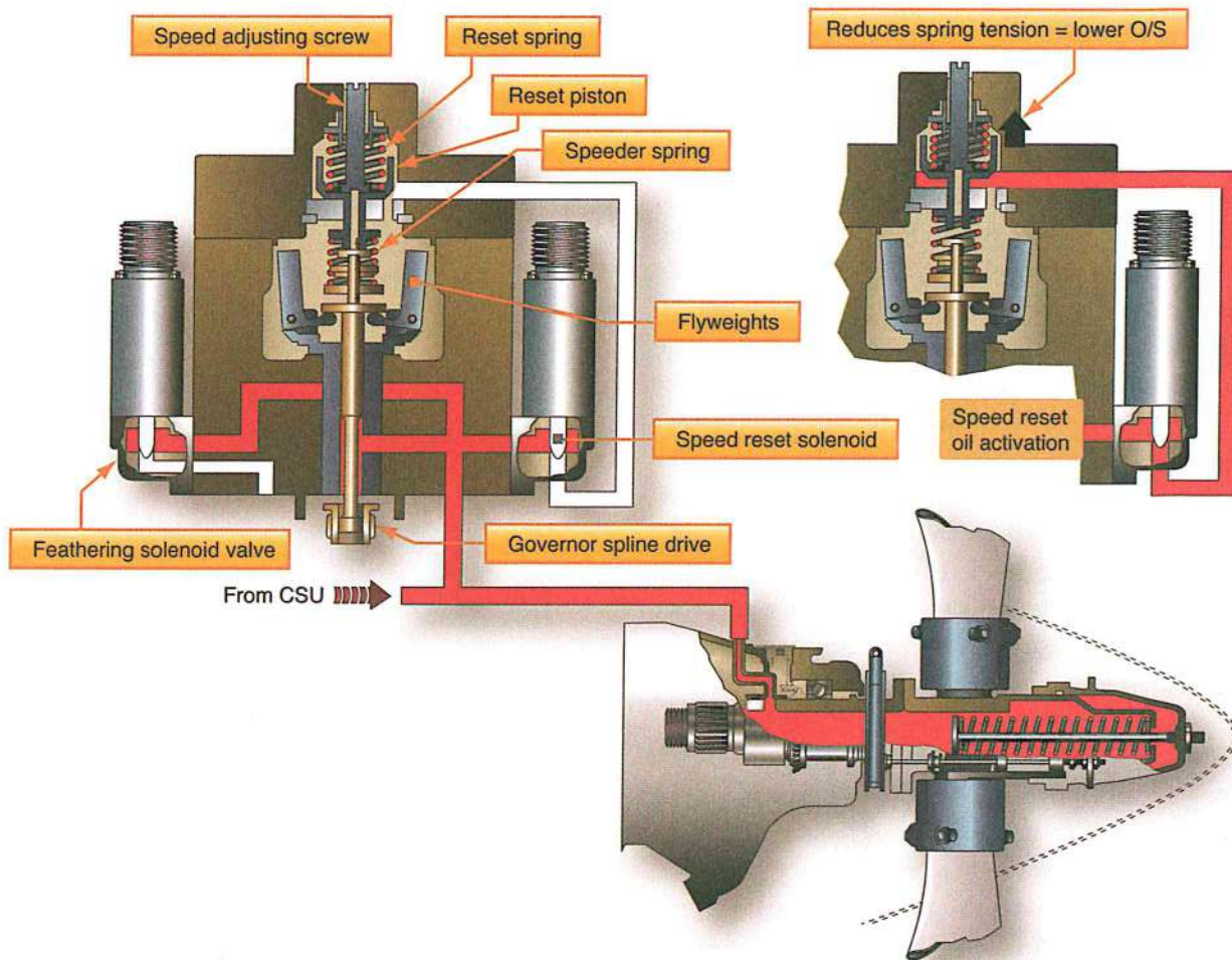
Figure 3-29. Over speed governor.
