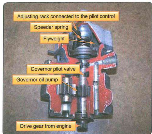
Figure 3-4. Internal workings of a propeller governor.
