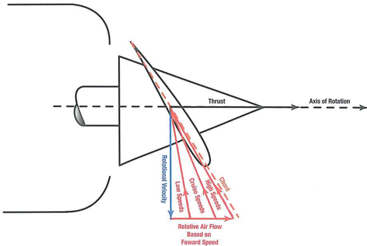
Figure 1-10. Relative air flow based on forward speed.
