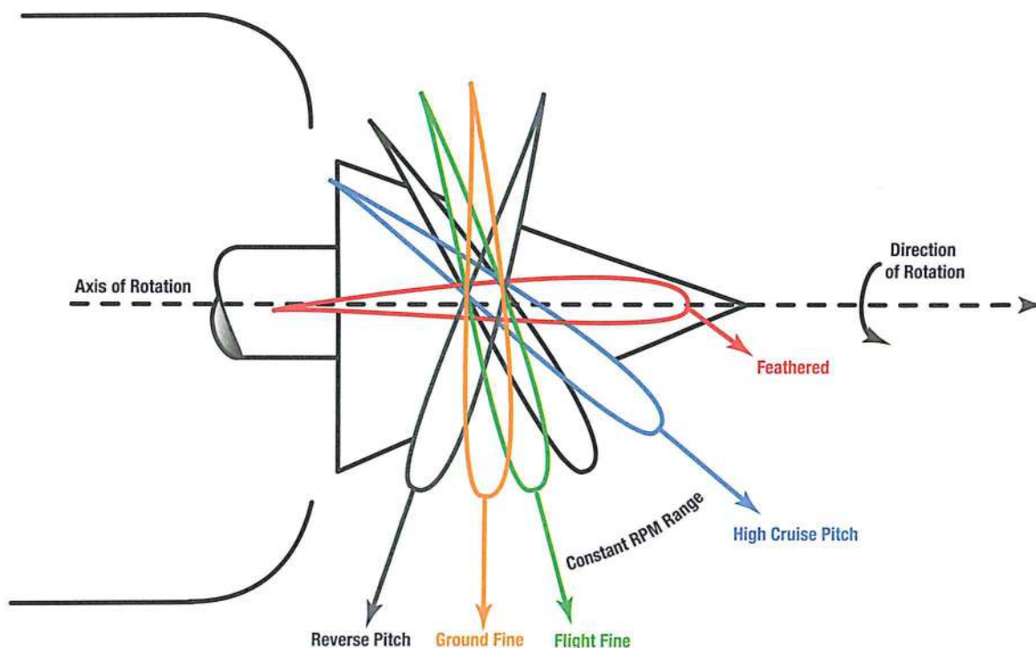
Figure 1-13. Range of propeller pitch for a variety of flight parameters.
