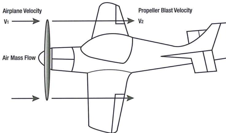
Figure 1-4. Thrust.
