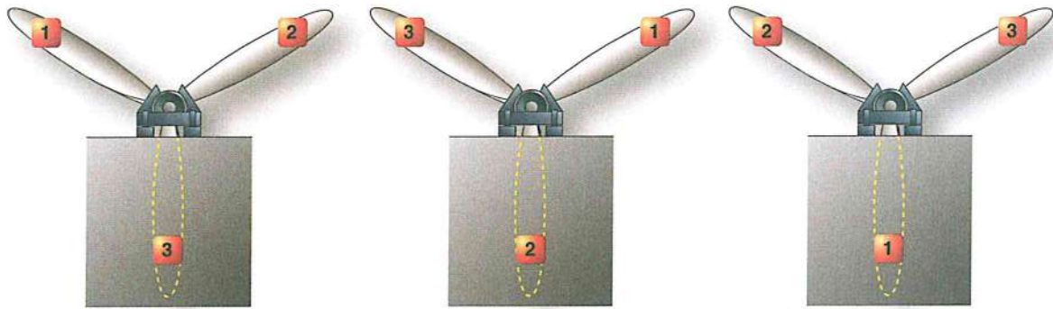
Figure 6-10. Checking three bladed propeller for static balance using knife-edge stand.
