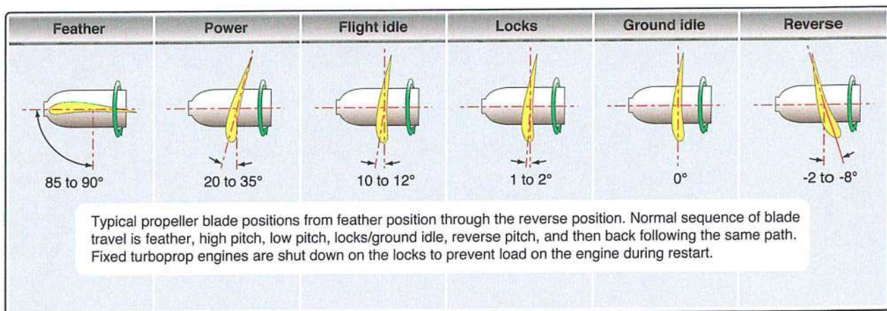
Figure 1-1. Ranges of Propeller Pitch.
