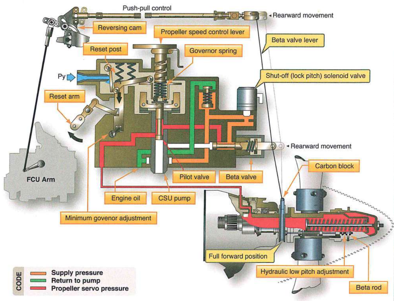
Figure 3-27. PT-6 Beta mode reverse operation.
