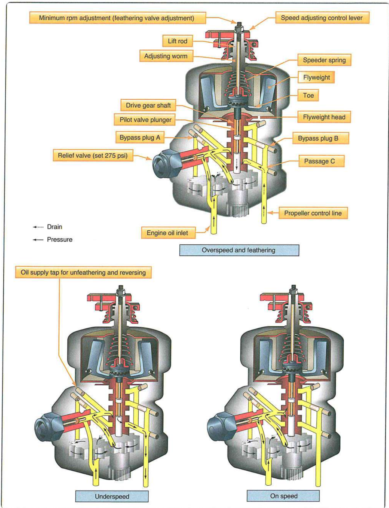
Figure 3-5. Propeller governor in over speed, under speed, and on speed conditions
