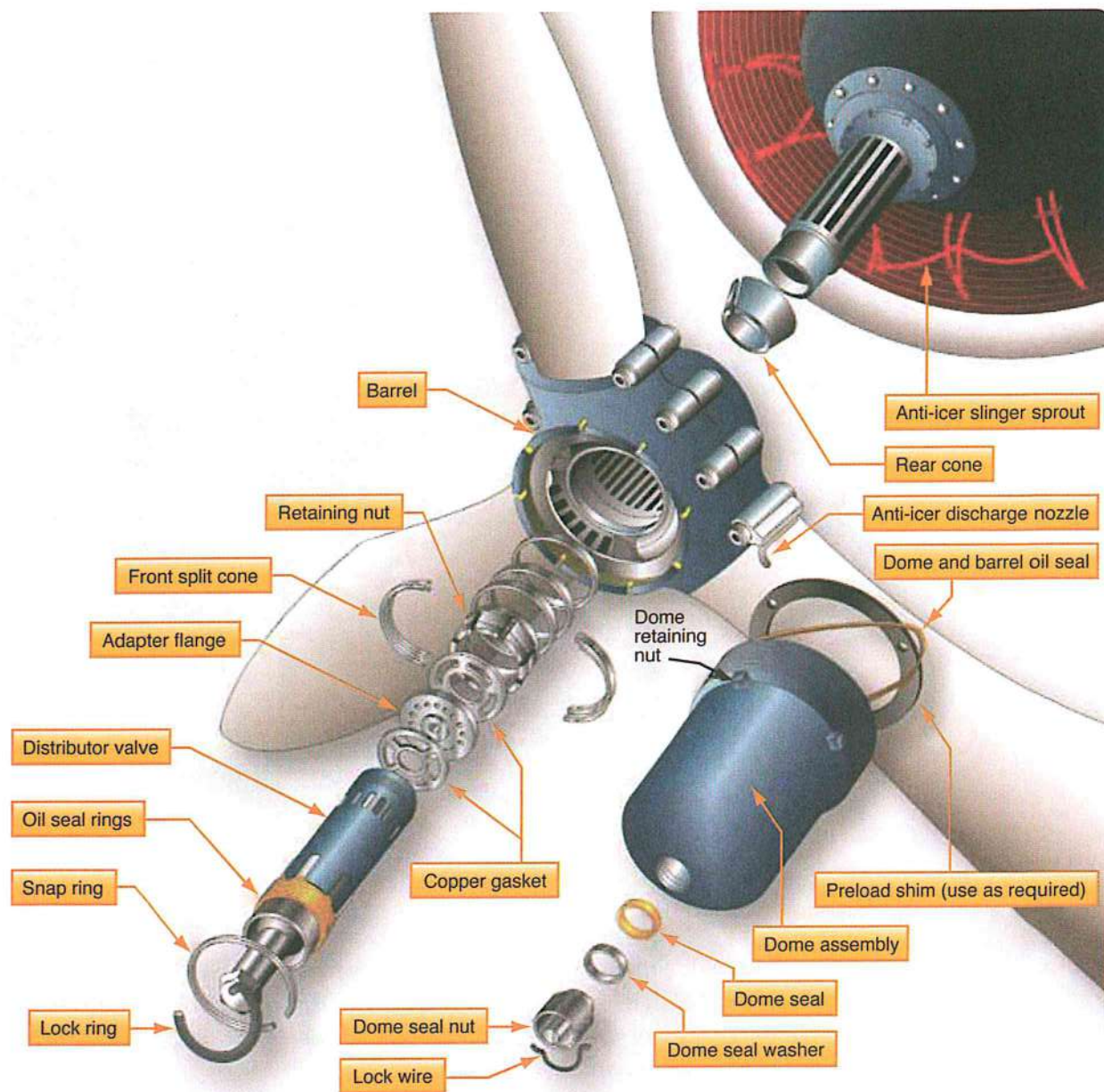
Figure 3-12. Hamilton Standard Hydromatic Propeller.
