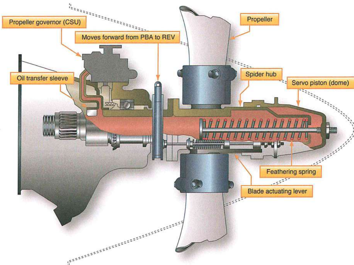
Figure 3-24. PT-6 Propeller pitch change cutaway.
