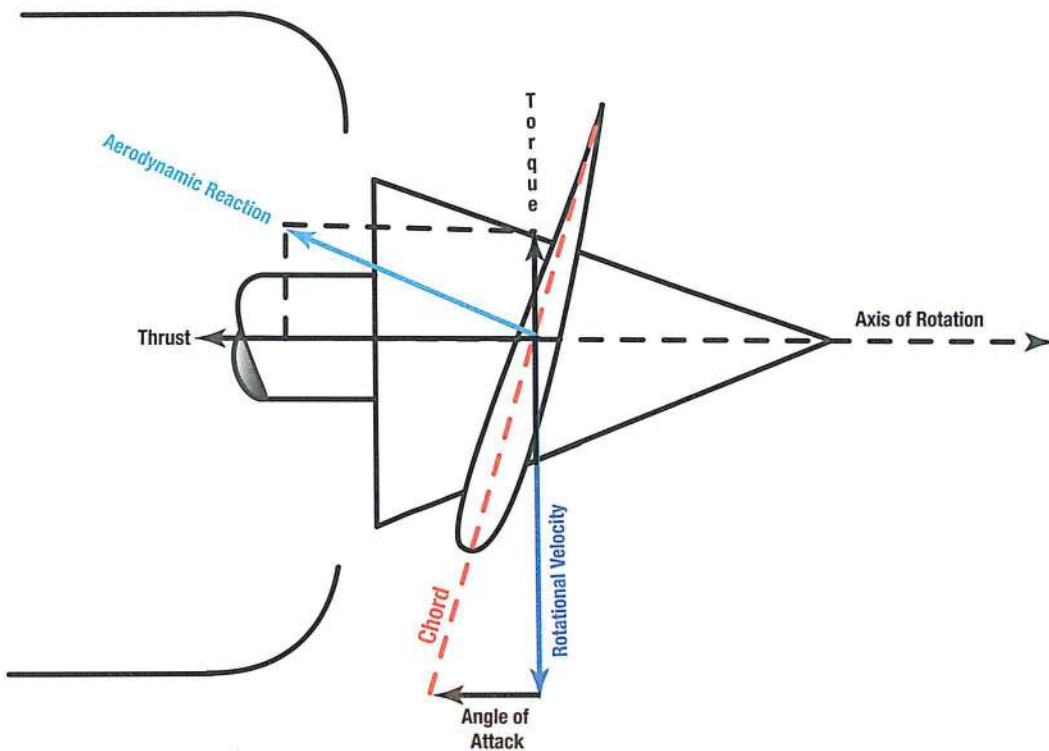
Figure 1-11. Reverse Thrust.
