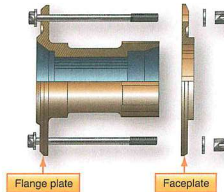
Figure 2-6. Wooden propeller hub adapter.
