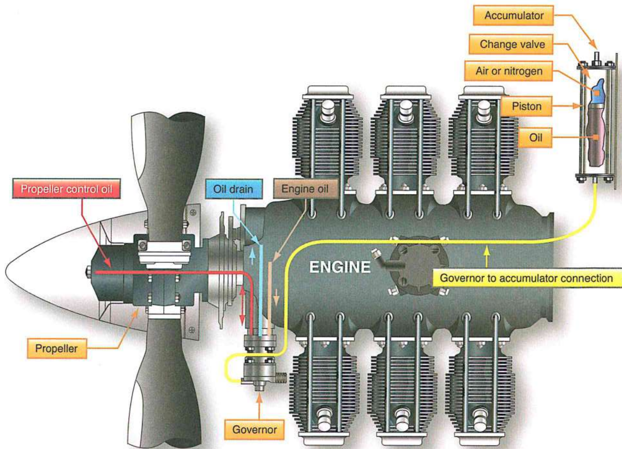
Figure 3-11. Unfeathering accumulator system.
