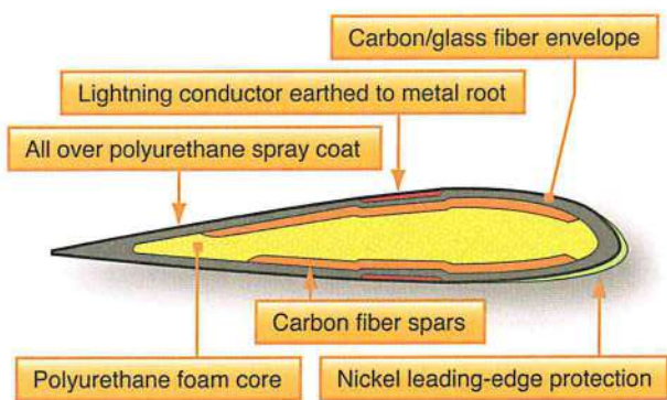
Figure 2-9. Makeup of composite propeller blade.
