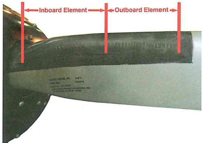
Figure 5-8. De-icing boots or overshoes.
