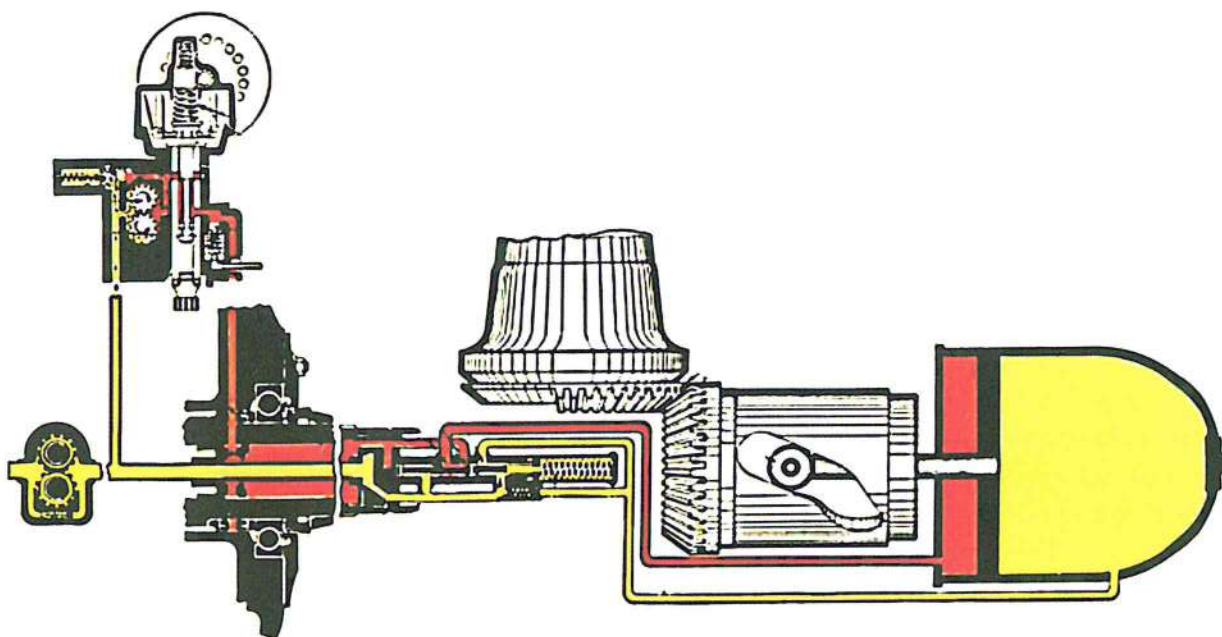
Figure 3-14. Hydromatic propeller in the on speed condition.
