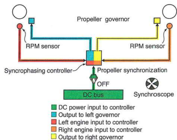
Figure 4-2. Propeller synchronizer and synchrophaser.
