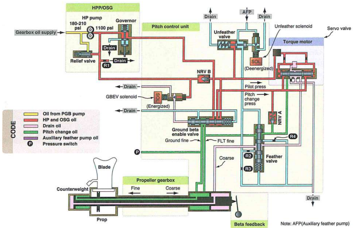
Figure 3-23. Propeller control system schematic.
