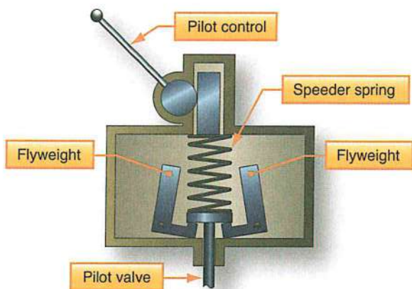
Figure 3-7. Propeller governor in an under speed condition.
