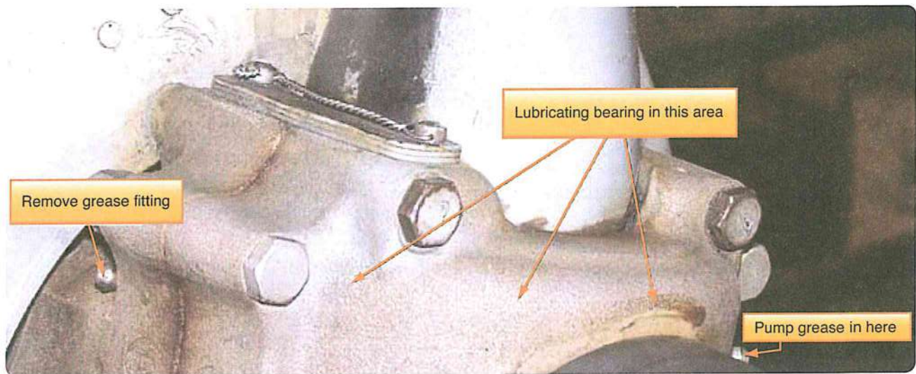
Figure 6-20. Sample lubrication points on propeller hub.
