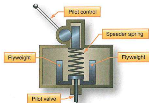
Figure 3-6. Propeller governor in an on speed condition. It should be pointed out that when the governor is installed on the engine, it is adjusted to establish an on speed condition when the engine is operating at redline rpm with the propeller control in the full increase rpm, or low pitch, position. Having the maximum engine rpm adjusted and maintained by the governor reduces the risk of the engine experiencing operations beyond the redline rpm.
