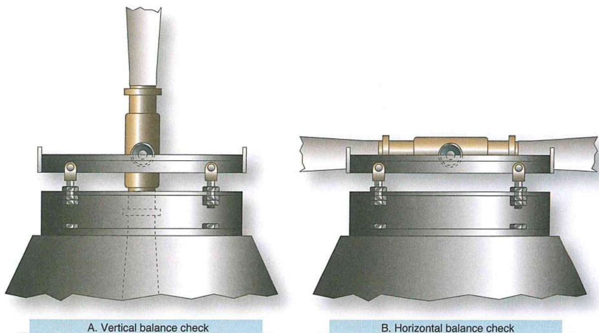
Figure 6-9. Checking two bladed propeller for static balance using knife-edge stand.
