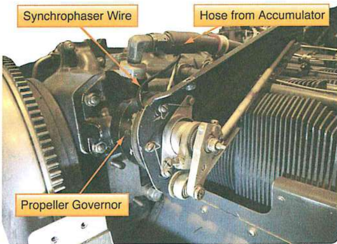
Figure 3-3. Propeller governor equipped with synchronization and synchrophaser system and hose from unfeathering accumulator (note wire and hose attached to the governor).
