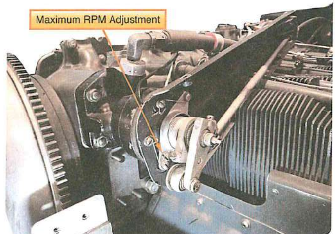
Figure 6-24. Propeller governor maximum rpm adjustment.
