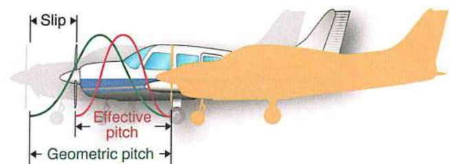
Figure 1-5. Effective Pitch versus Geometric Pitch.
