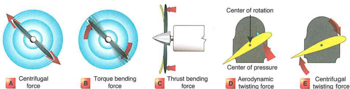
Figure 1-14. Forces acting on a propeller.
