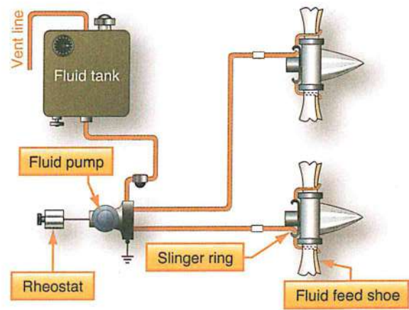
Figure 5-2. Fluid anti-ice system.
