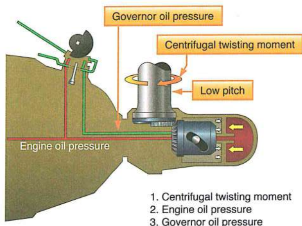
Figure 3-13. Hydromatic operational forces.
