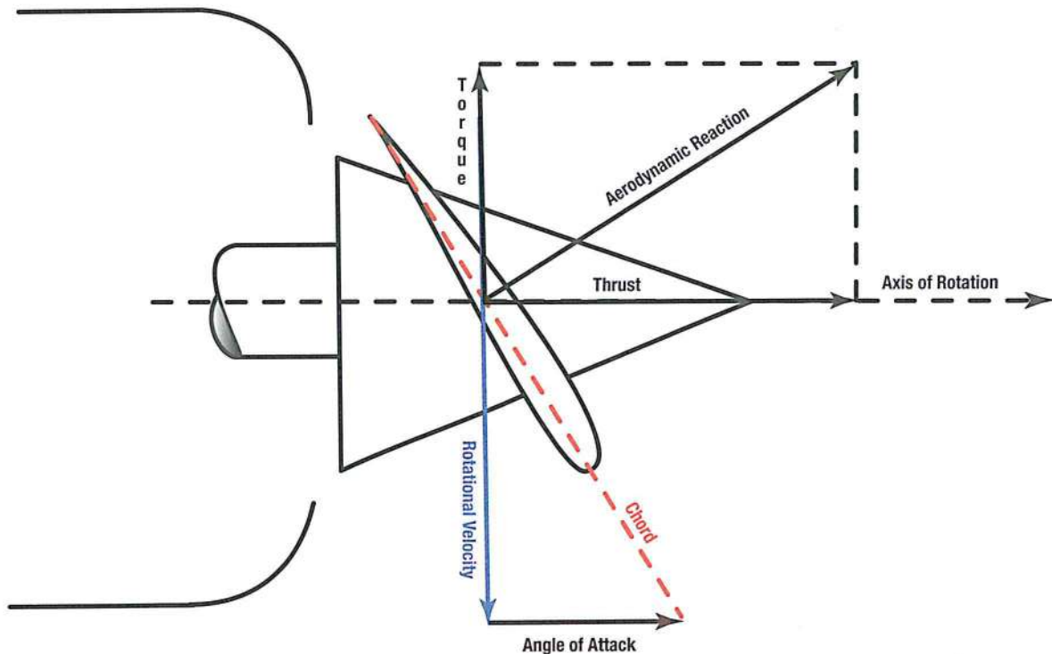
Figure 1-9. Propeller blade angle with no forward airspeed.
