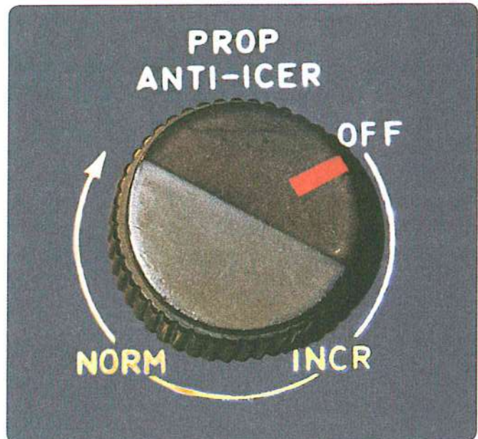
Figure 5-11. Rheostat control on anti-ice with variable flow.
