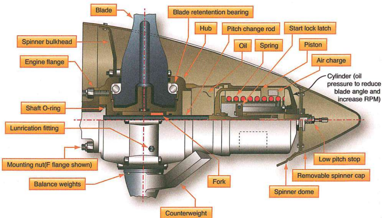
Figure 3-10. Constant speed, feathering propeller.
