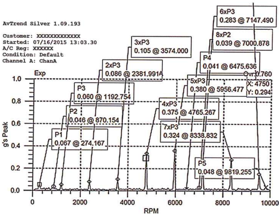
Figure 6-19. Sample vibration spectrum survey.
