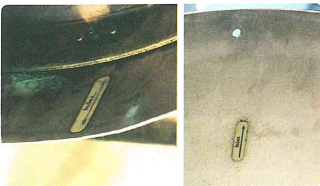
Figure 2-20. Index mark on spinner bulkhead shown on left image and index mark on spinner shown on right image. Technicians should align the two marks before installing the spinner.
