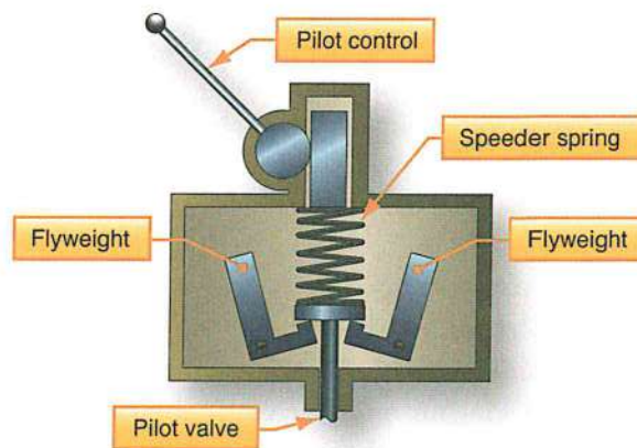
Figure 3-8. Propeller governor in an over speed condition.
