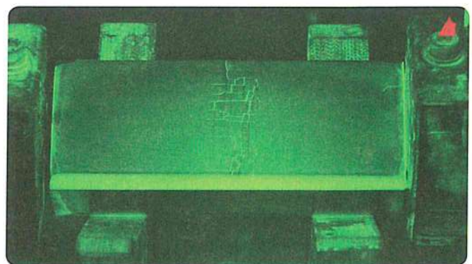
Figure 6-2. Cracking within a ferrous metal as revealed by magnetic particle inspection.
