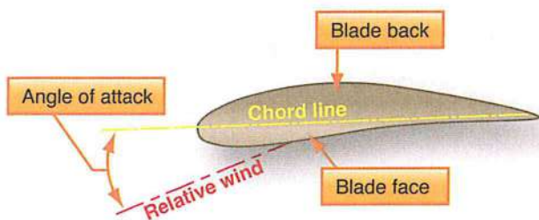
Figure 1-3. Cross Section of Propeller Airfoil.
