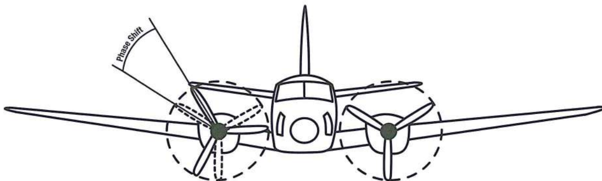
Figure 4-5. Propeller phase altered by synchrophaser.
