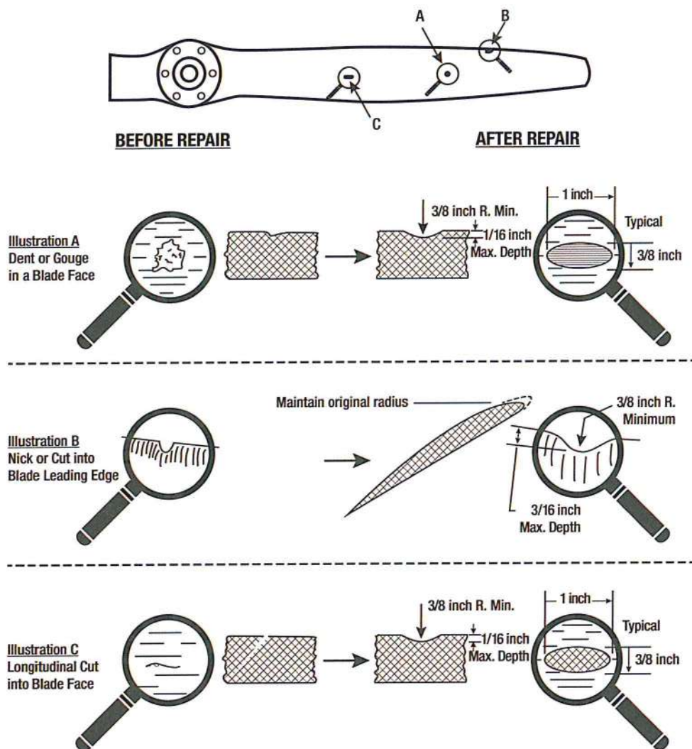
Figure 6-23. Examples of dressing defects from propeller blades.
