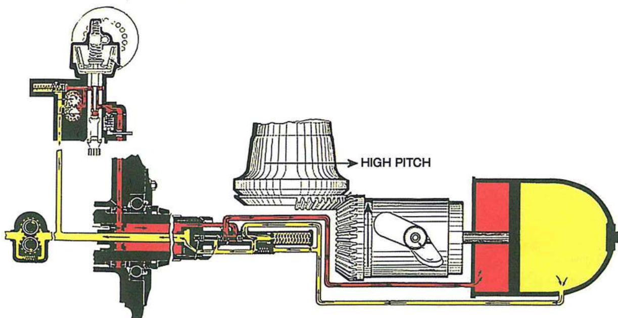
Figure 3-16. Hydromatic propeller in the over speed condition.
