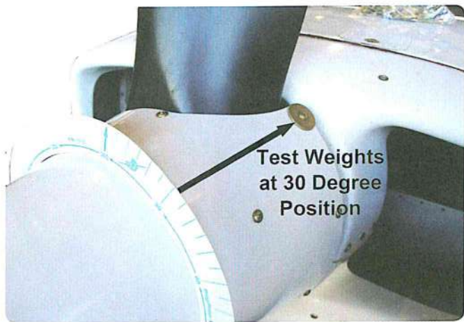
Figure 6-14. Using special protractor to determine location in reference to 12 O'Clock blade, test weight is added to spinner screw. DO NOT FLY aircraft with test weights installed. Analyzer will calculate new weight package for permanent installation location on spinner bulkhead.
