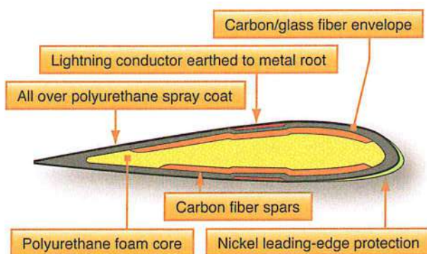
Figure 6-3. Composite propeller blade cross section.
