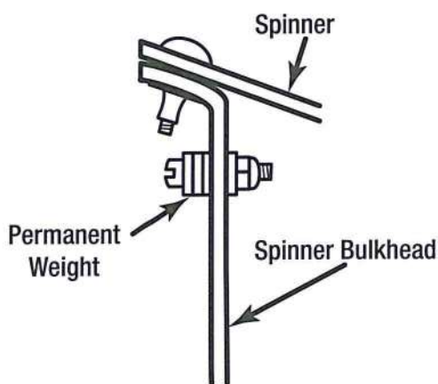
Figure 6-15. Sample permanent weight installation on spinner bulkhead.
