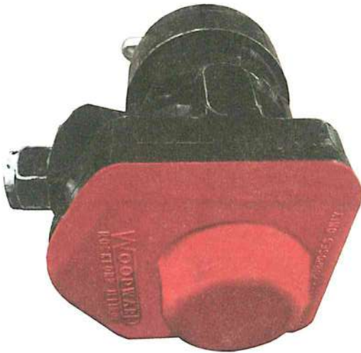
Figure 7-2. Protective cap placed on propeller governor mounting surface. Used for shipping and storage.
