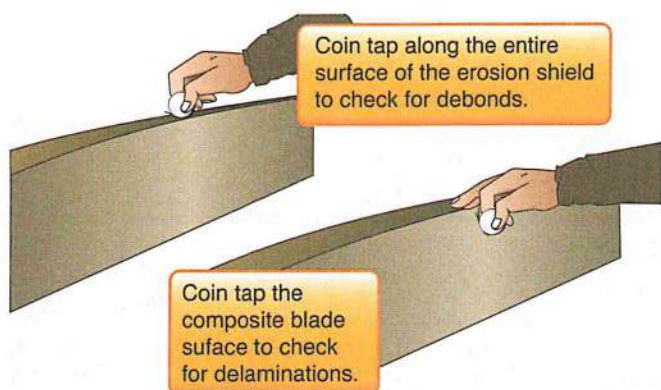
Figure 6-4. Checking composite propeller blade using coin tap test.
