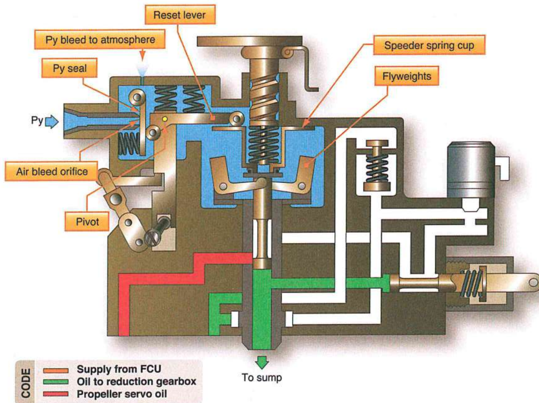
Figure 3-28: Nf (Engine over speed) governor.
