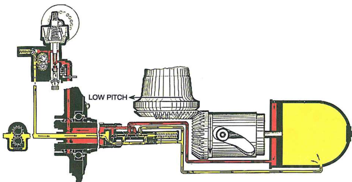
Figure 3-15. Hydromatic propeller in the under speed condition.
