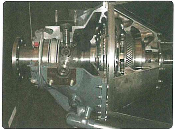
Figure 3-21. Turboprop gear reduction box.
