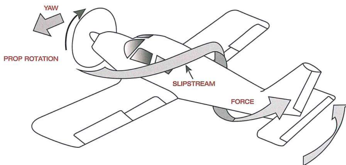
Figure 1-16. Slipstream Effect.
