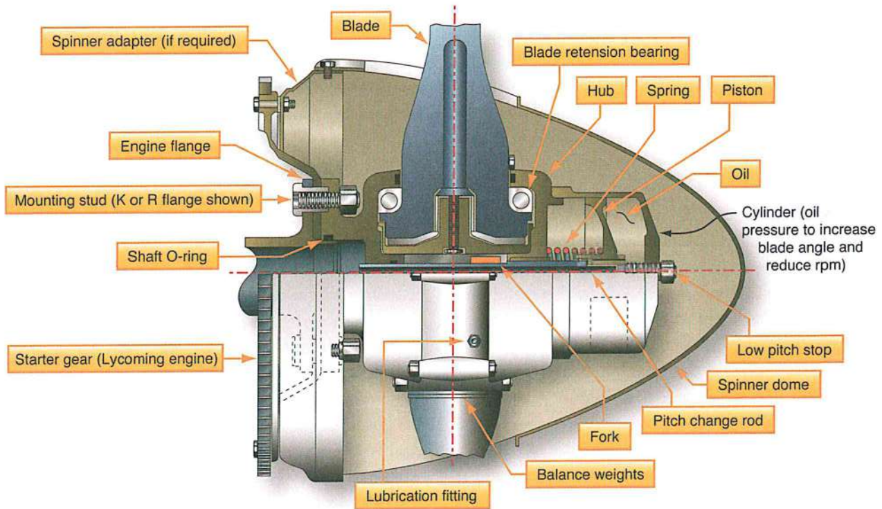
Figure 3-9. Constant speed, non-feathering propeller.
