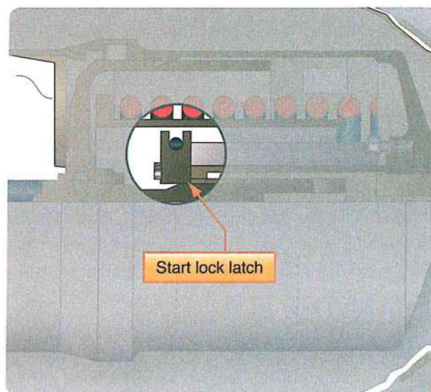
Figure 2-16. Feathering latch.
