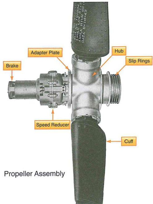
Figure 3-30. Curtiss-Wright electrically controlled propeller.
