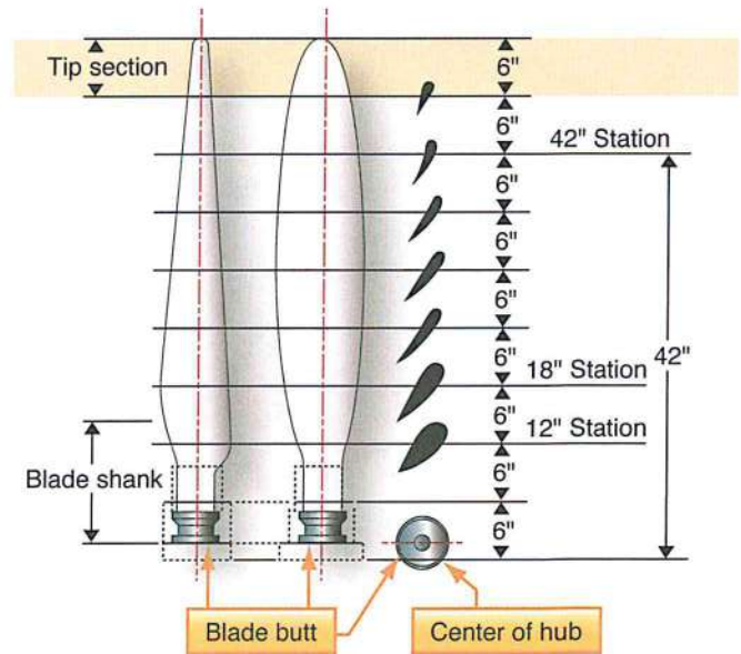
Figure 1-7. Propeller blade elements demonstrating twist.
