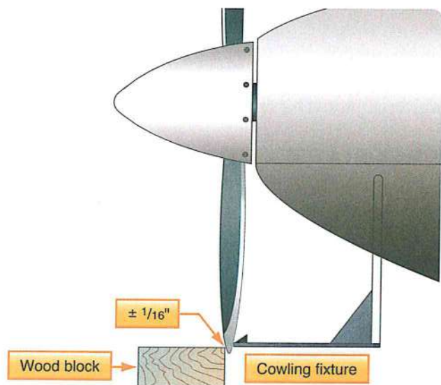
Figure 6-5. Checking propeller blade track.
