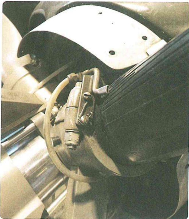
Figure 5-4. Propeller anti-ice discharge nozzle and blade boot.
