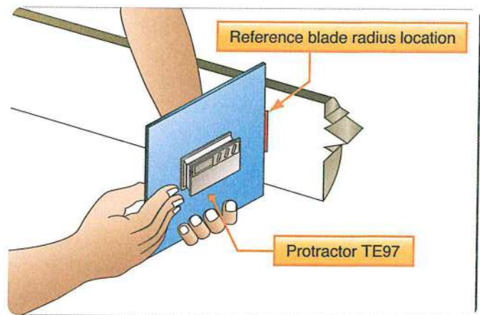
Figure 6-7. Blade angle measurement with handheld protractor.
