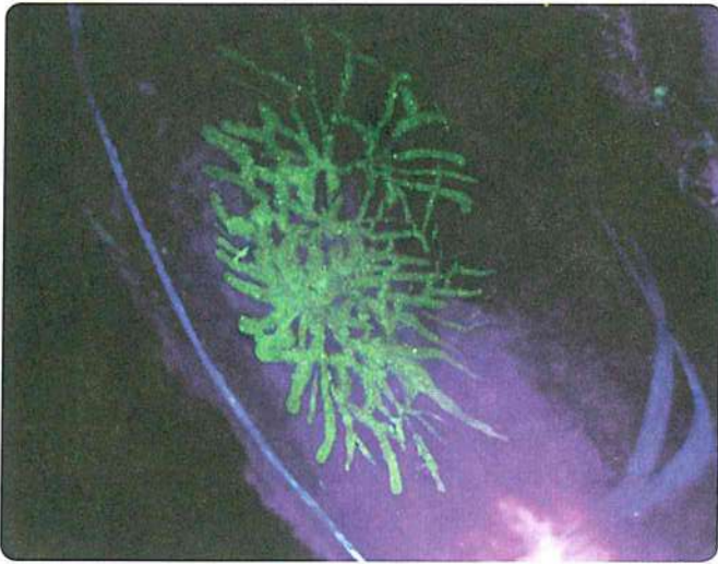
Figure 6-1. Stress corrosion cracking as revealed by fluorescent liquid penetrant inspection.
