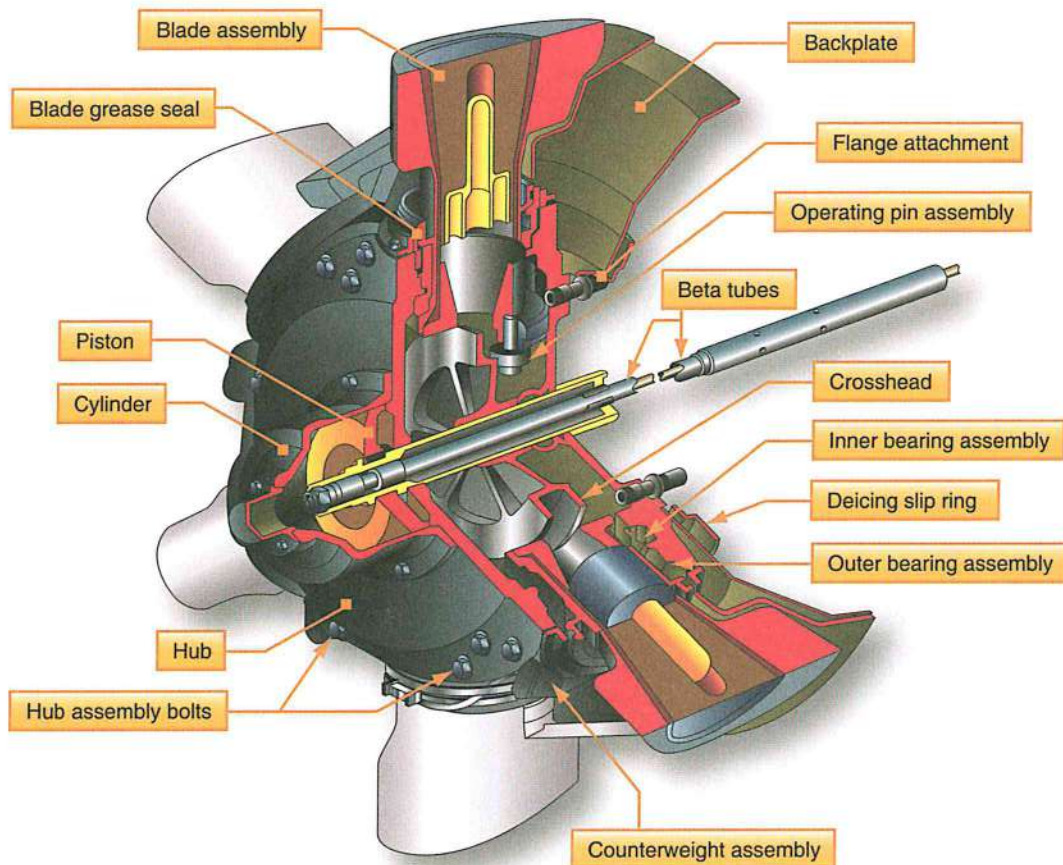
Figure 3-22. Cutaway turboprop propeller.
