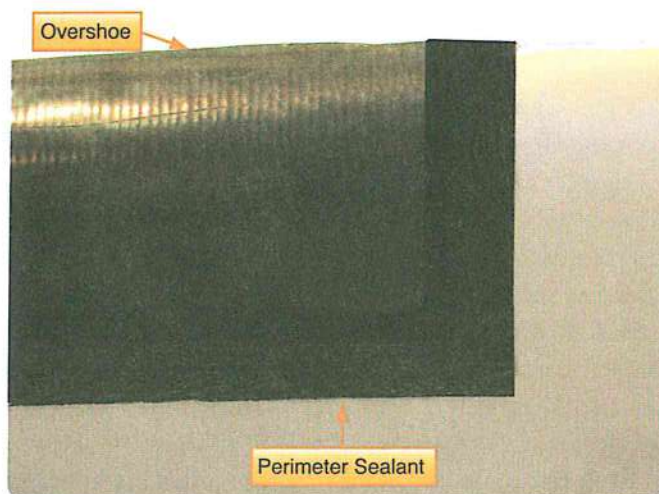
Figure 5-13. Sealant applied to overshoe perimeter.
