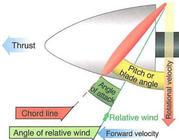
Figure 1-6. Propeller Aerodynamics.
