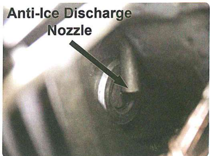
Figure 5-3. Anti-ice fluid discharge into slinger ring.
